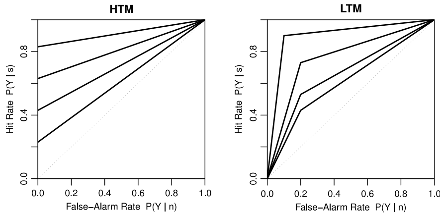
Fig. 1. Examples of ROCs as predicted by the HTM and LTM.
