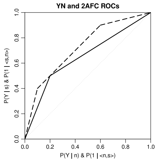
Fig. 4. Example of YN and 2AFC ROC (solid and dashed lines, respectively) as predicted by the LTM with parameters q_s = 0.50 and q_n = 0.20 .
